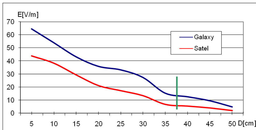
Fig. 5. The E electric field strength measurement results in the ELF frequency range for the Galaxy 520 and the Satel CA 64 control panels
