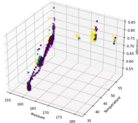
Fig. 7. 3D scatter plot showing the interaction between pressure (PS1), temperature (TS1), and vibration (VS1) across different fault classes
