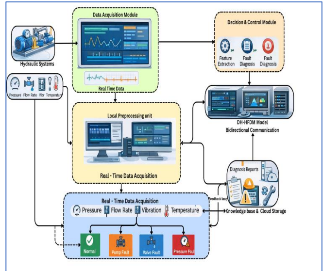
Fig. 2. Real-time deployment and operational workflow of the drl-hfdm model
