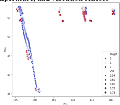
Fig. 6. Multi-sensor scatter plot illustrating the relationship between PS1 and TS1, with VS1
