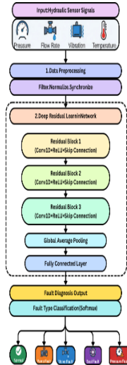
Fig. 1. Architecture of the proposed drl-hfdm model for hydraulic fault detection
