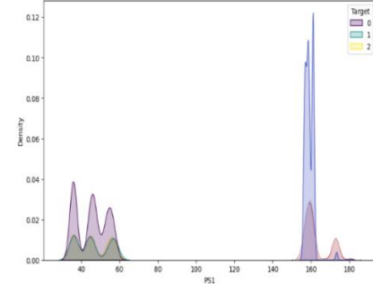
Fig. 3. Density distribution of PS1 sensor values for different fault conditions
