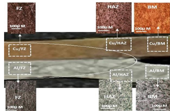
Fig. 19. RSW zones of the Al-Cu Joint
