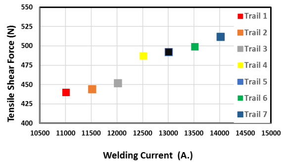
Fig. 12. Effect of welding current on RSW tensile shear force
