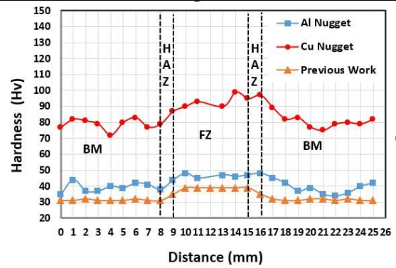
Fig. 18. Micro-hardness for RSW Joints as compared with Ref. [51], thick. = 1 mm
