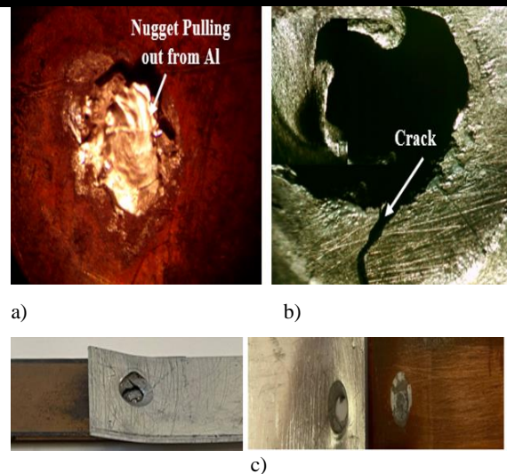
Fig. 15. PF modes in Al-Cu RSW: a) Cu side pull out the Al-nugget side, 10 x; b) Al-nugget side, 10 x; c) Cu and Al nugget after failure
