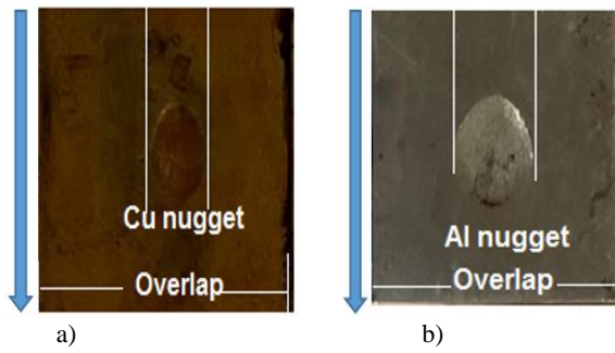
Fig. 16. Welded joints: a) Cu-weld nugget; b) Al-weld nugget
