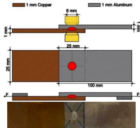
Fig. 5. RSW specimen dimensions
