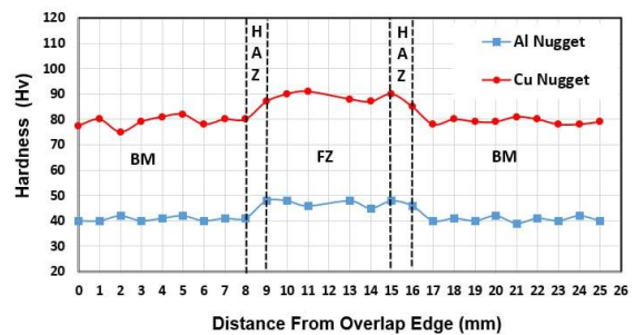
Fig. 17. Surface hardness for RSW joint
