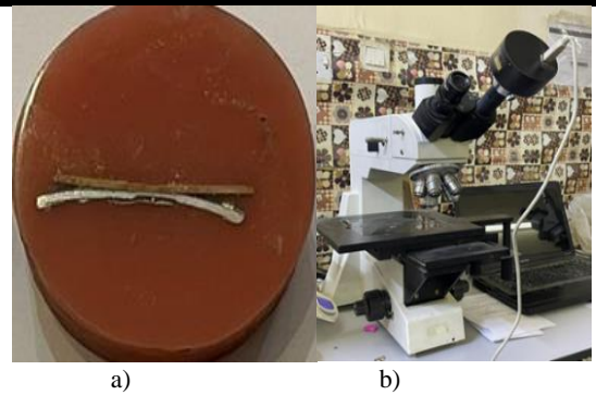
Fig. 10. a) Embedded sample; b) Microscopic device [10]
