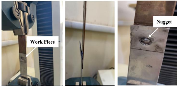
Fig. 13. Tensile test for welded joints
