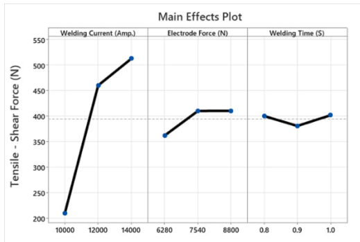
Fig. 3. Main effects plot of tensile force
