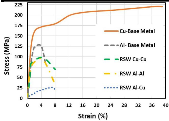
Fig. 11. Stress with strain curve for pre-weld metals and post-weld joints. Al-1050, and pure Cu
