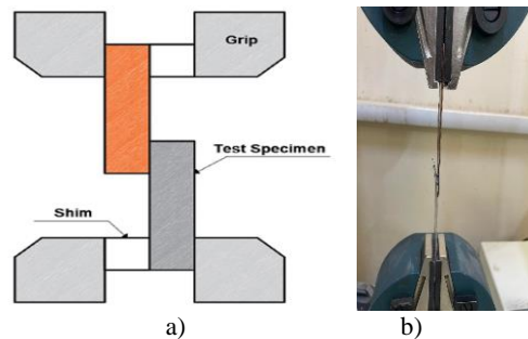
Fig. 6. Tensile shear test: a) Schematic of the specimens with Shims; b) Specimens gripped
