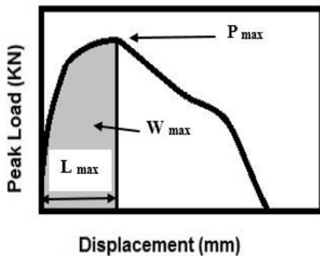
Fig. 1. Load-displacement curve in a tensile test; W_{max} : energy absorption; P_{max} : peak load; L_{max} : elongation at peak load [25]
