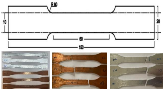
Fig. 4. Tensile-shear specimens and dimensions
