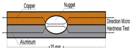
Fig. 9. Cross-section micro hardness
