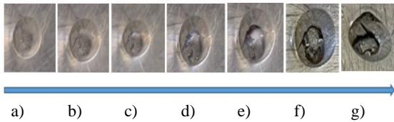
Fig. 14. Initiation with propagation of crack in tensile shear test during consecutive time periods: a) 0 min; b) 1 min; c) 2 min; d) 3 min; e) 4 min; f) 5 min; g) final failure mode
