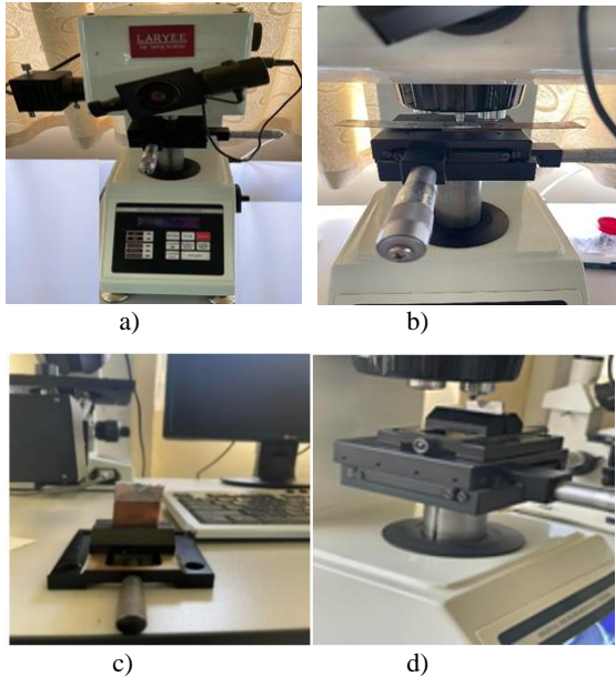
Fig. 8. a) Vickers Micro Hardness Testing device; b) Surface Micro Hardness Measurement for RSW Joint; c) Cross-Section Micro Hardness Specimen with Special Grip; d) Cross-Section Micro hardness measurement
