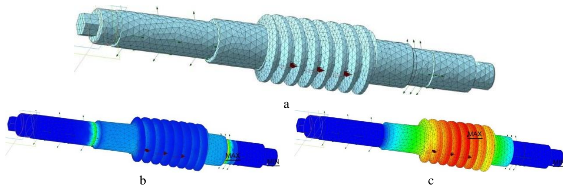
Fig. 2. Finite-element analysis of the worm: a – finite-element mesh, supports, and loading; b – stress fields; c – displacement fields
