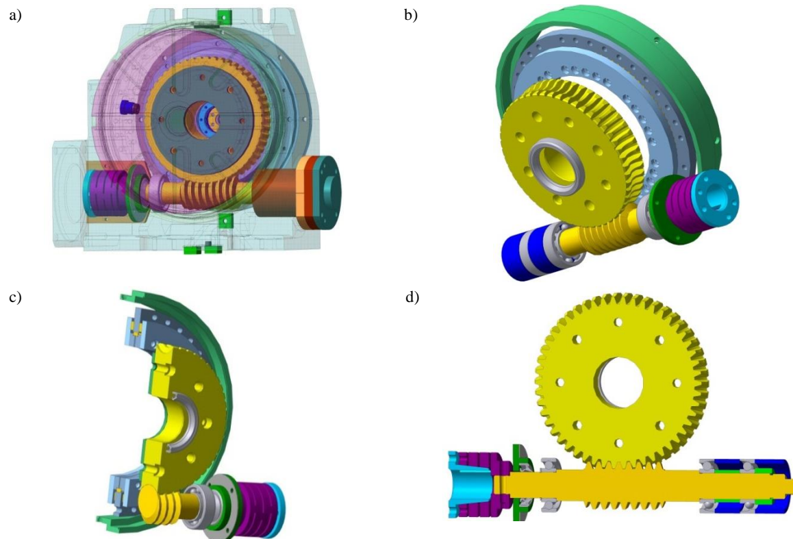
Fig. 1. A three-dimensional model of a rotary table with a faceplate: a – general view with the option of transparency; b – worm transmission; c, d – sections of the worm gear with a special bearing
