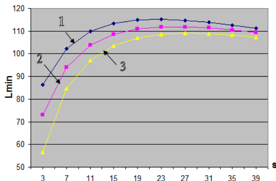
Fig. 4. The effect of the shifting coefficient x on the value L_{\Sigma \min} : curve 1 ( x = -1 ); curve 2 ( x = 0 ); curve 3 ( x = +1 )
