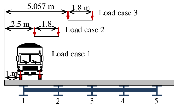
Fig. 7. Vehicle loading
