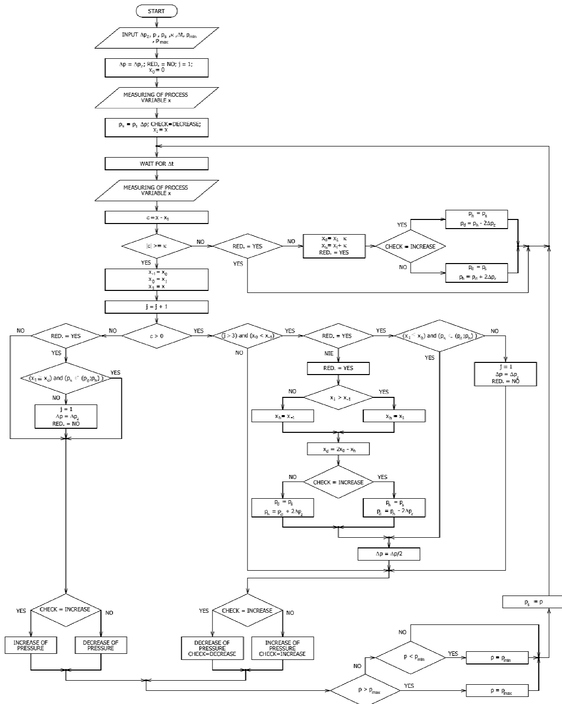
Fig.5. Algorithm of extremal control
