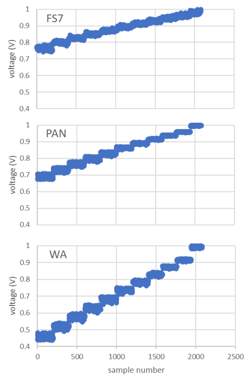
Fig. 12. Flow sensors 20 s window measured values
