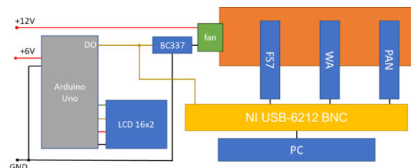
Fig. 7. Measure scheme
