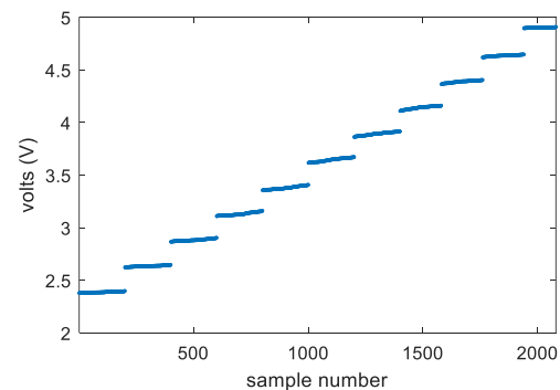
Fig. 9. PWN signal (real data from 20 s analyse window)
