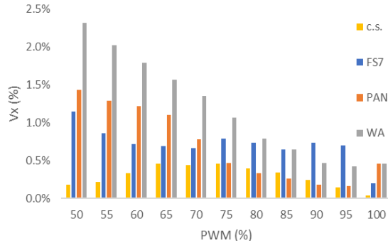
Fig. 14 Coefficient of variation for tested sensors
